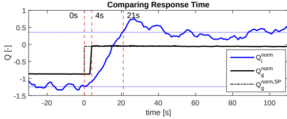
Figure 9: Step response. The initial and final mean values of Q_l are also indicated. The values were normalized for facilitating the visualization. We step the gas injection setpoint at 0 s. The control takes 4 s to track the new setpoint, while the system settles at a new steady-state after approximately 20 s.
