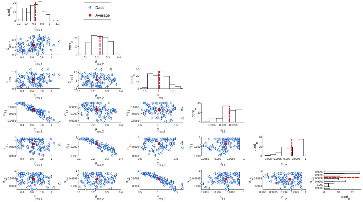
Figure 15: 100 independent steady-state model adaptation runs using historical data. The histograms of the individual parameters are plotted, with a red line indicating the mean. Also, we show the 2-dimensional distribution, analyzing two parameters at a time. In these plots we also the average (red dot).
