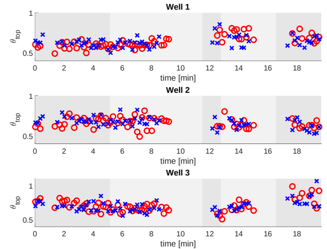
(b) Estimated parameter - scaled top valve coefficient.
