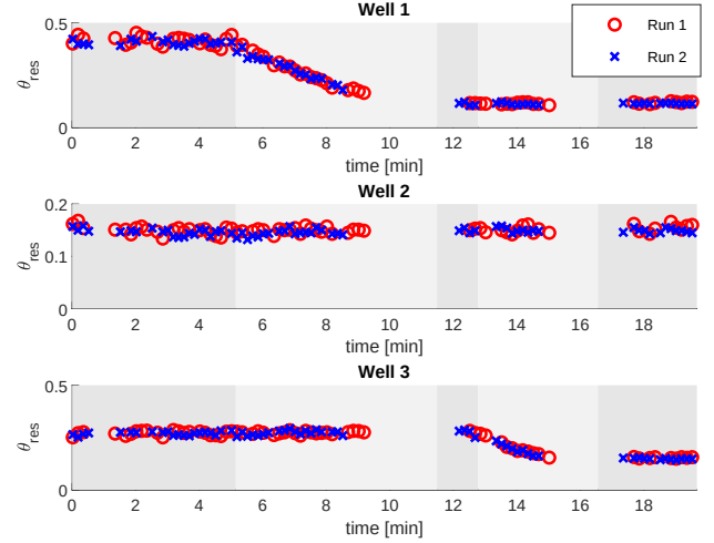
(a) Estimated parameter - scaled reservoir valve coefficient.
