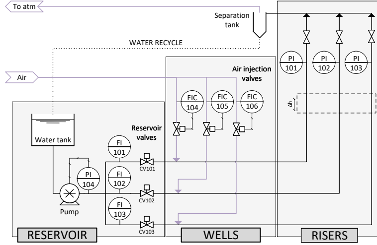
Figure 4: Experiment schematic. The system measurements y_p are the well top pressures (PI101, PI102 and PI103), the pump outlet pressure (PI104), the liquid flowrates (FI101, FI102, and FI103), and the gas flowrates (FI104, FI105, and FI106). Three PI controllers are used for controlling the gas flowrates, whose setpoints are the system inputs u computed by the optimization layer. The reservoir valve openings (CV101, CV102, and CV103) are the system disturbances. They change during the experiments for representing different reservoir behaviors, while the pump outlet pressure is kept constant by a PI controller.
