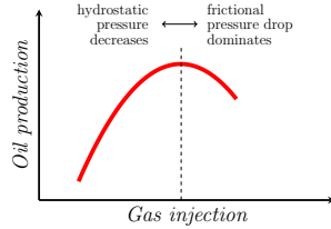
Figure 3: Gas lift effect on well's oil production. The dashed line indicates the turning point, in which the frictional pressure drop effect starts to dominate the hydrostatic pressure.
