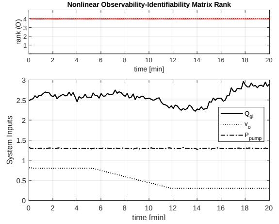
Figure 8: Nonlinear observability-identifiability matrix rank along the trajectory of a previous production optimization experiment based on steady-state RTO.
